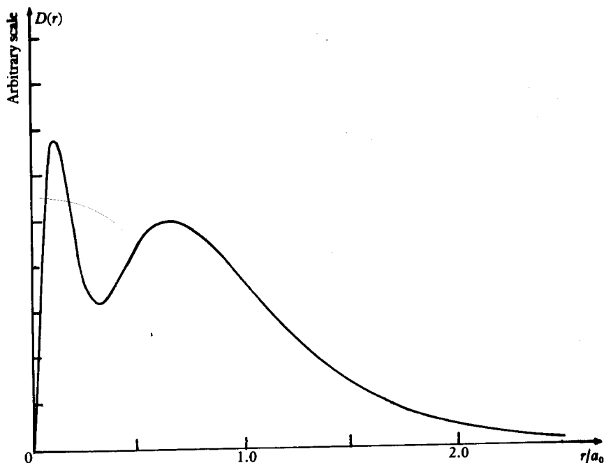
7.6 The radial density function D(r) for neon.
